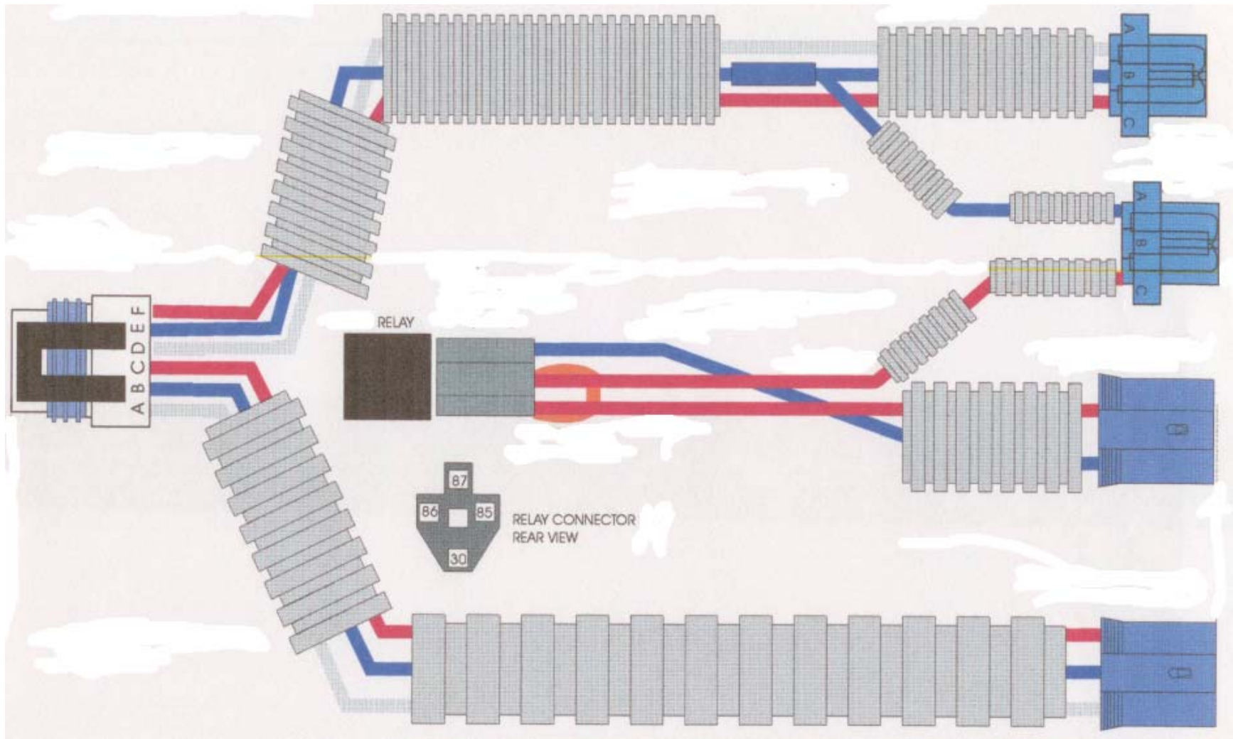
07221 Adapter Harness
