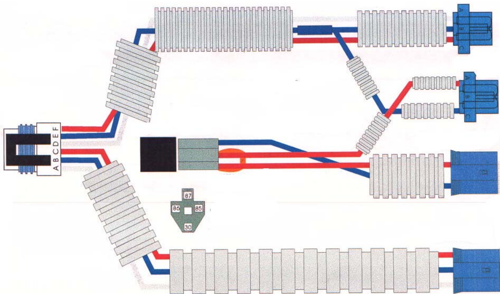
07190 Adapter Harness
