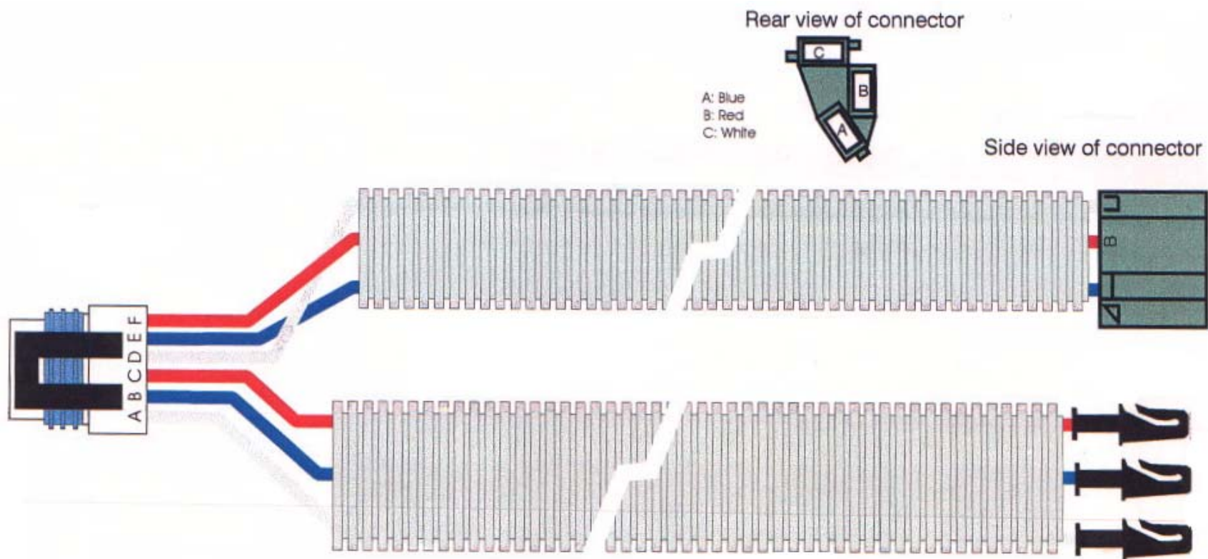
07105 Adapter Harness
