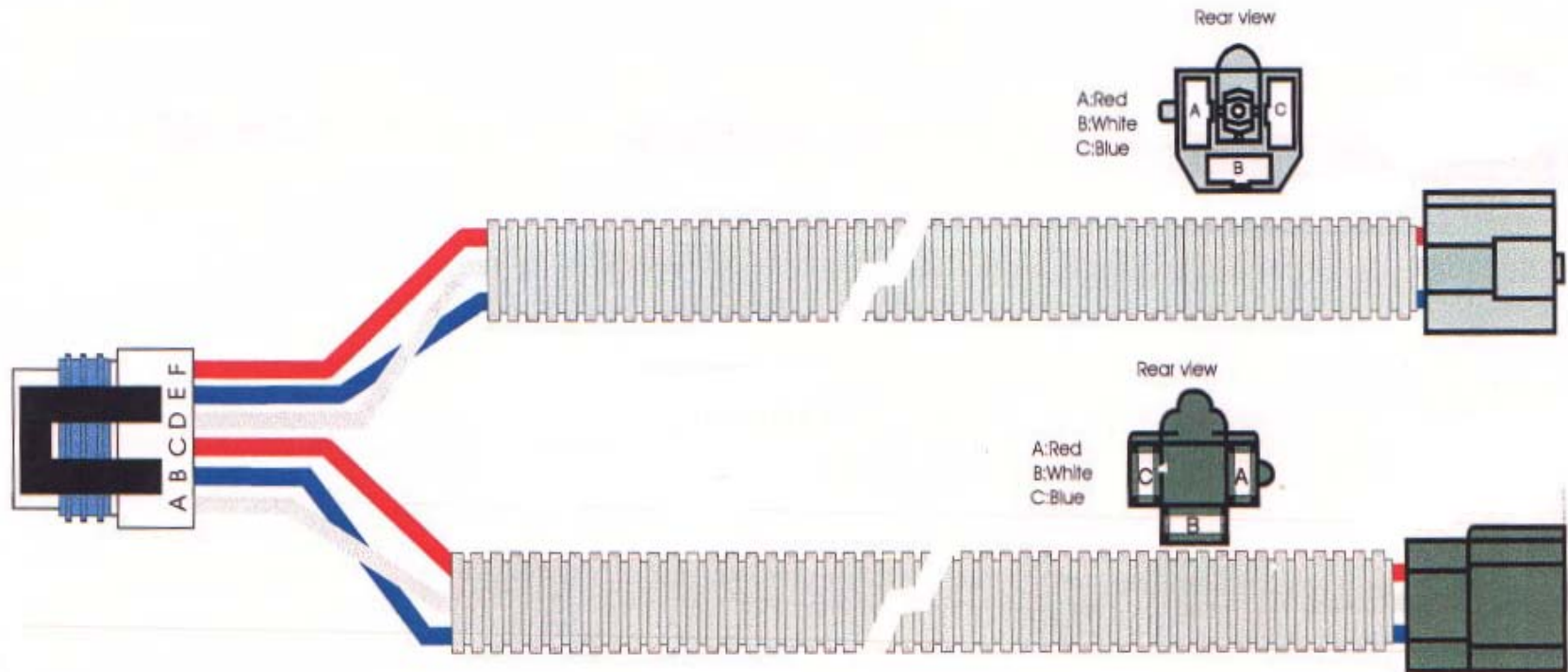
07099 Adapter Harness
