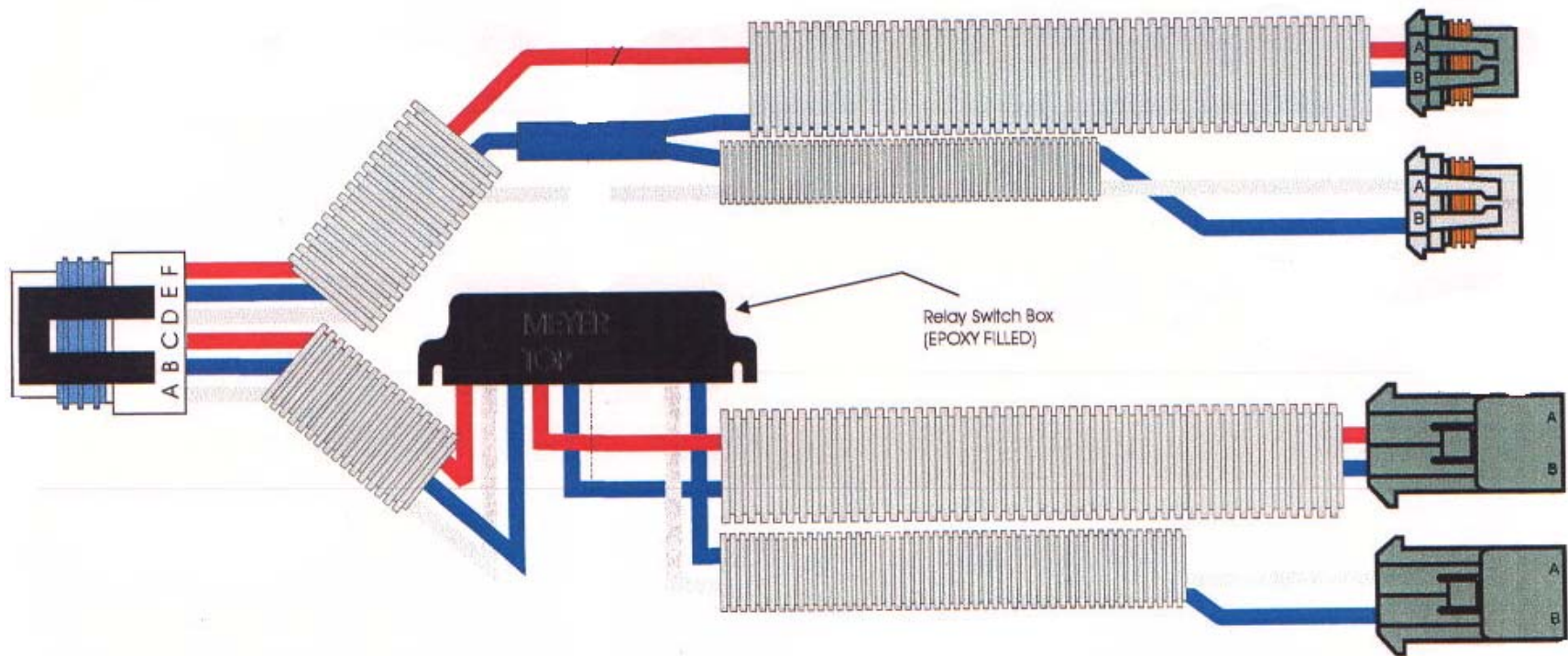
07213 Adapter Harness
