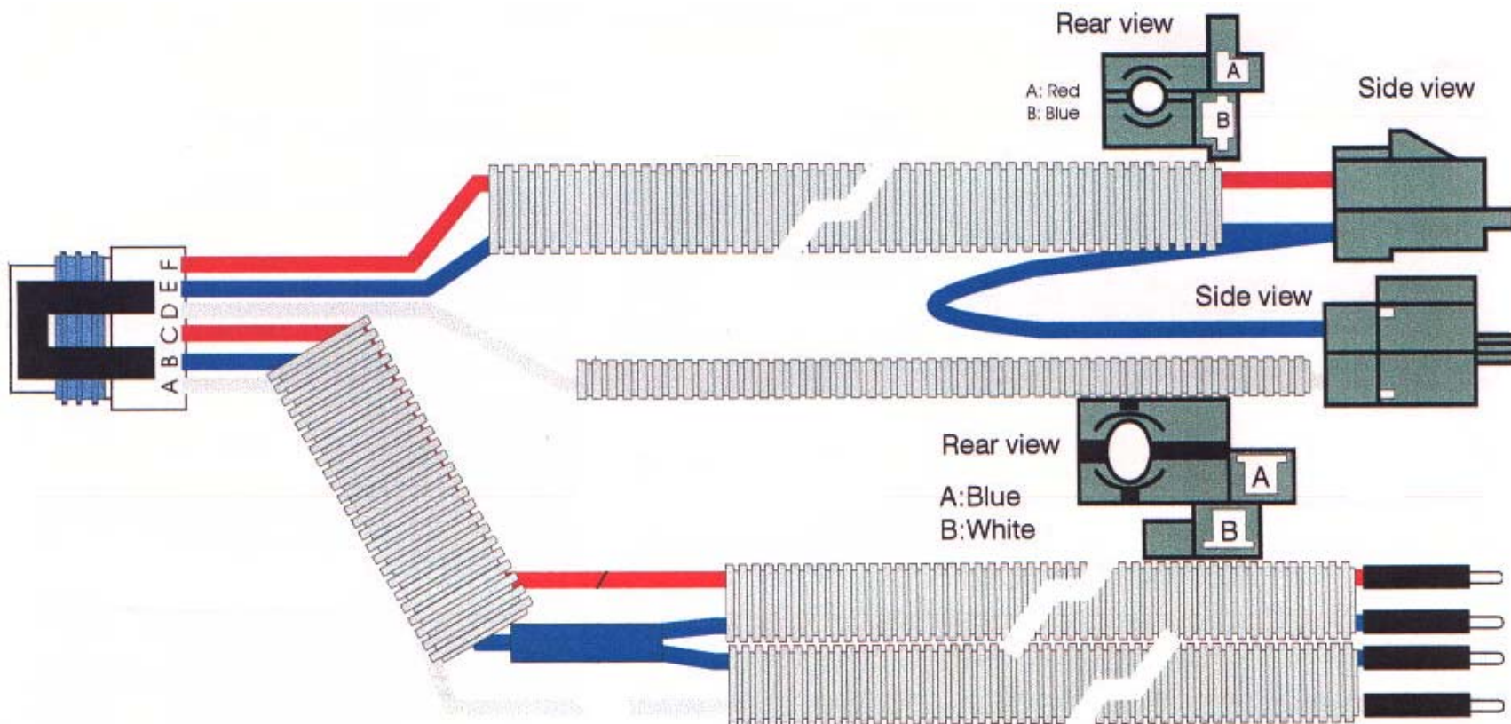
07103 Adapter Harness
